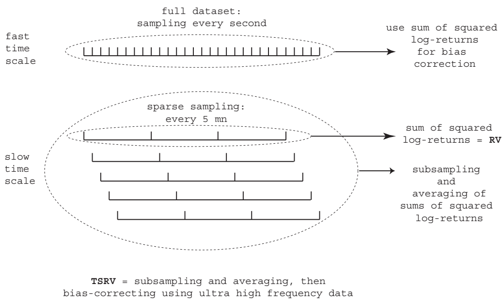
Fig. 3. This figure describes the construction of the TSRV estimator.
