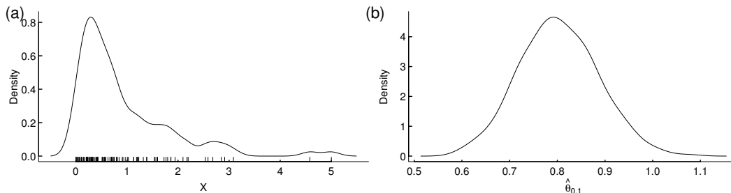
(a) Estimated density of the observations X_1, \dots, X_{100} and (b) estimated sampling distribution of the trimmed mean \hat{\theta}_{0.1} (based on B = 1000 bootstrap replications).
